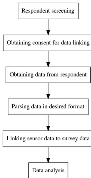
Figure 4: Sensor data linking process
